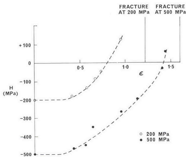
FIG. 4. The variation of resultant triaxial stress component at the centre of the neck ( H ) with natural strain ( \epsilon ) for specimens strained at 200 and 500 MPa.
